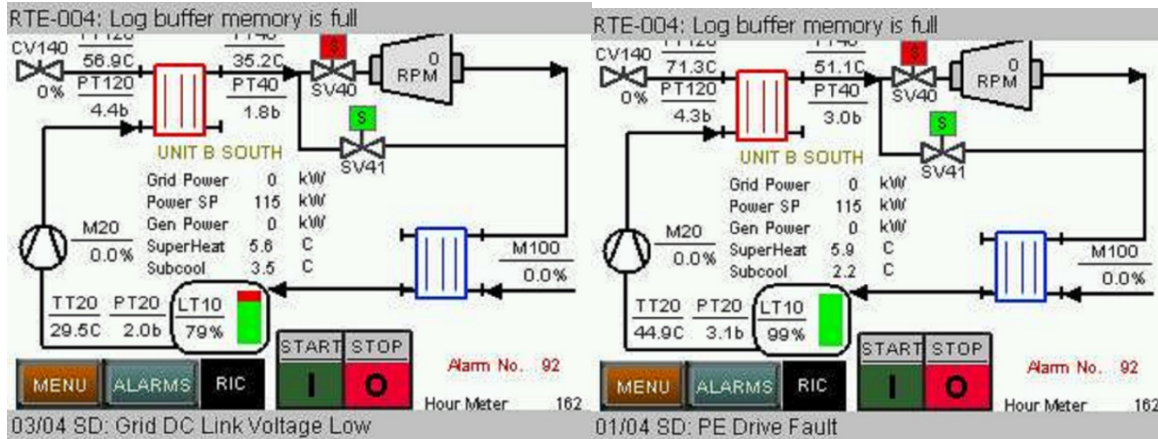
Figure 1.8. Screen shot of south unit during operation. (TT120 = Geothermal fluid temperature (°C), PT120 = Geothermal fluid pressure (bars); TT20 = Working fluid inlet temperature (°C); PT40 = Working fluid inlet pressure (bars); TT50 = Working fluid exhaust temperature (°C))
