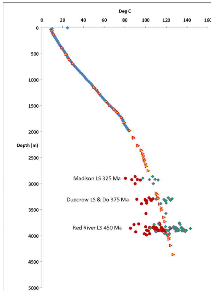
Figure 2.2 Demonstration of TSTRAT. An equilibrium temperature vs depth plot, blue line, is overlain by temperatures calculated by TSTRAT on formation tops, red-gold triangles. BHT data from wells within 10 km of the observation well, red dots, were corrected with the Kehle correction 18 , green diamonds, which tends to under correct at shallow depths and over correct at greater depths.
